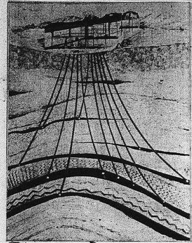
WHIP-STOCK DRILLING—Diagram shows whipstock method of well drilling to be employed on 7 acre oil lease granted by the city last night. From central site, exploratory drilling may be done in any direction or in any depth.
