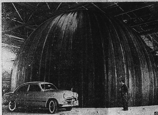
TO MEET ARCTIC WEATHER CONDITIONS—A new type inflated radar dome, built of rubber and fiber glass by Goodrich for the U. S. Air Force, will house aircraft warning equipment in the Arctic. The dome is 27 feet high and can withstand 125-mile-an-hour winds.
